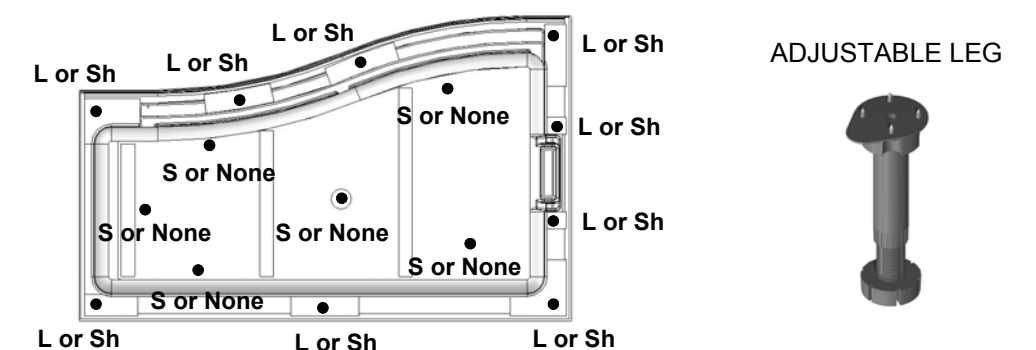
Figure 1: Tray Leg Positions for Wave with Side Panel & Alcove (Alcove tray shown in illustration)
